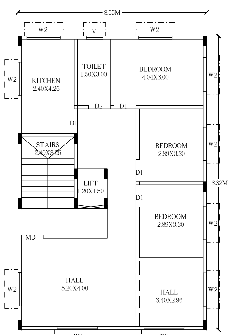
EXISTING FIRST FLOOR WITH ALTERATIONS
